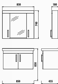
Wall Hung Star 85 Set
