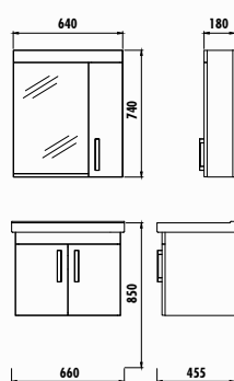
Wall Hung Star 65 Set
