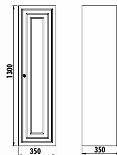
Kayra High Cabinet
