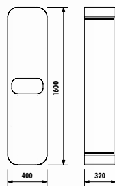
Pion High Cabinet
