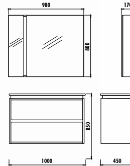
Verti 100 Set (with Drawer)
