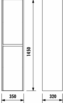
Link High Cabinet
