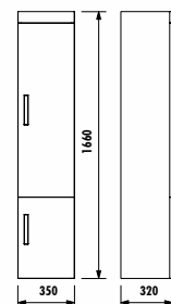
Wall Hung Star High Cabinet
